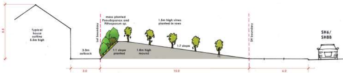
Long Section through vine planting 1:150 @A3
