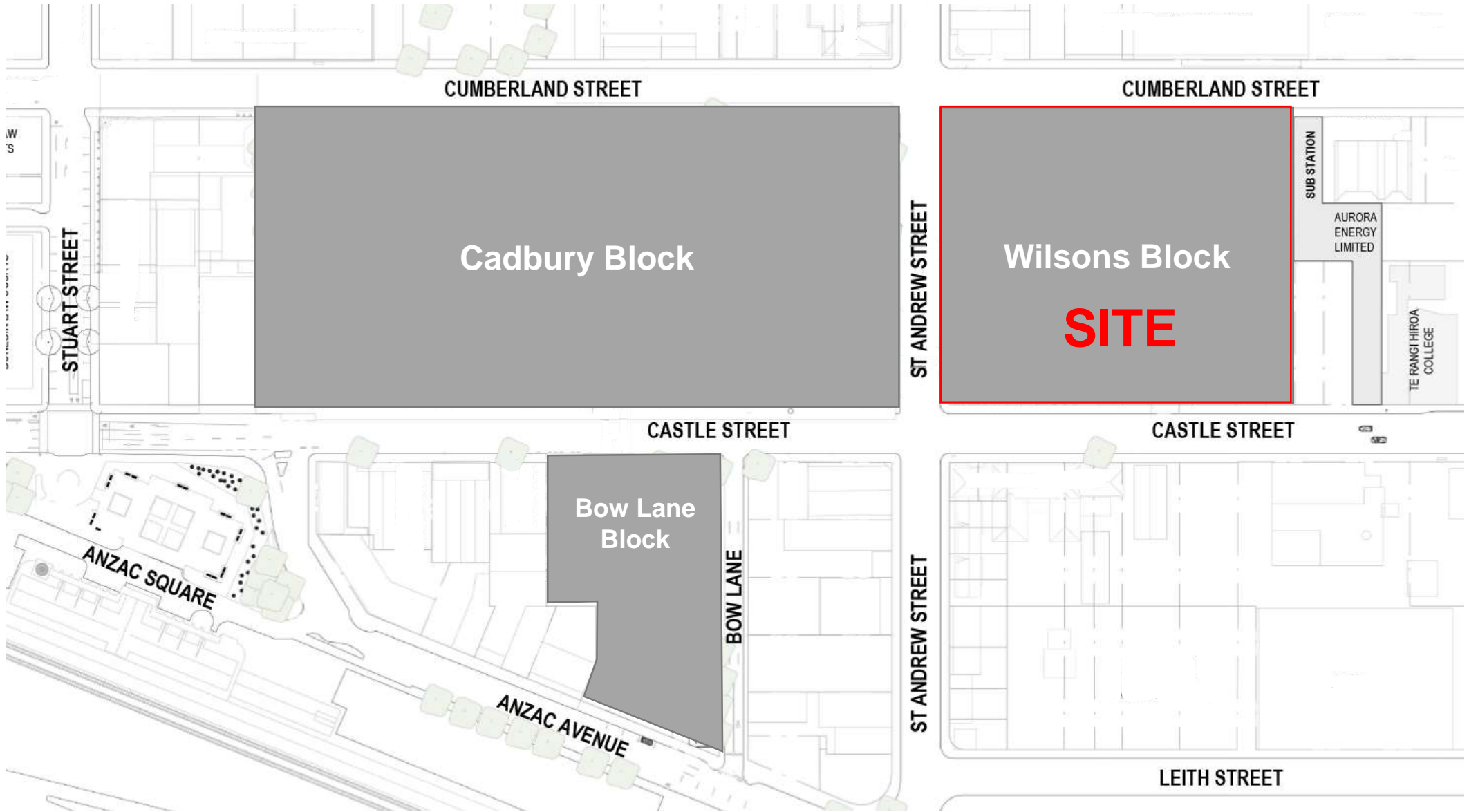
NDH - Overall Site Plan
