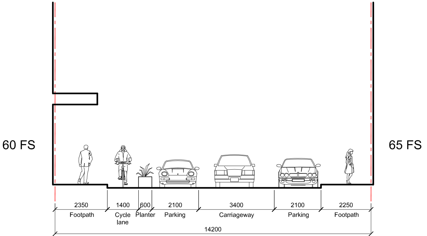
1 Existing Street and Existing Building
