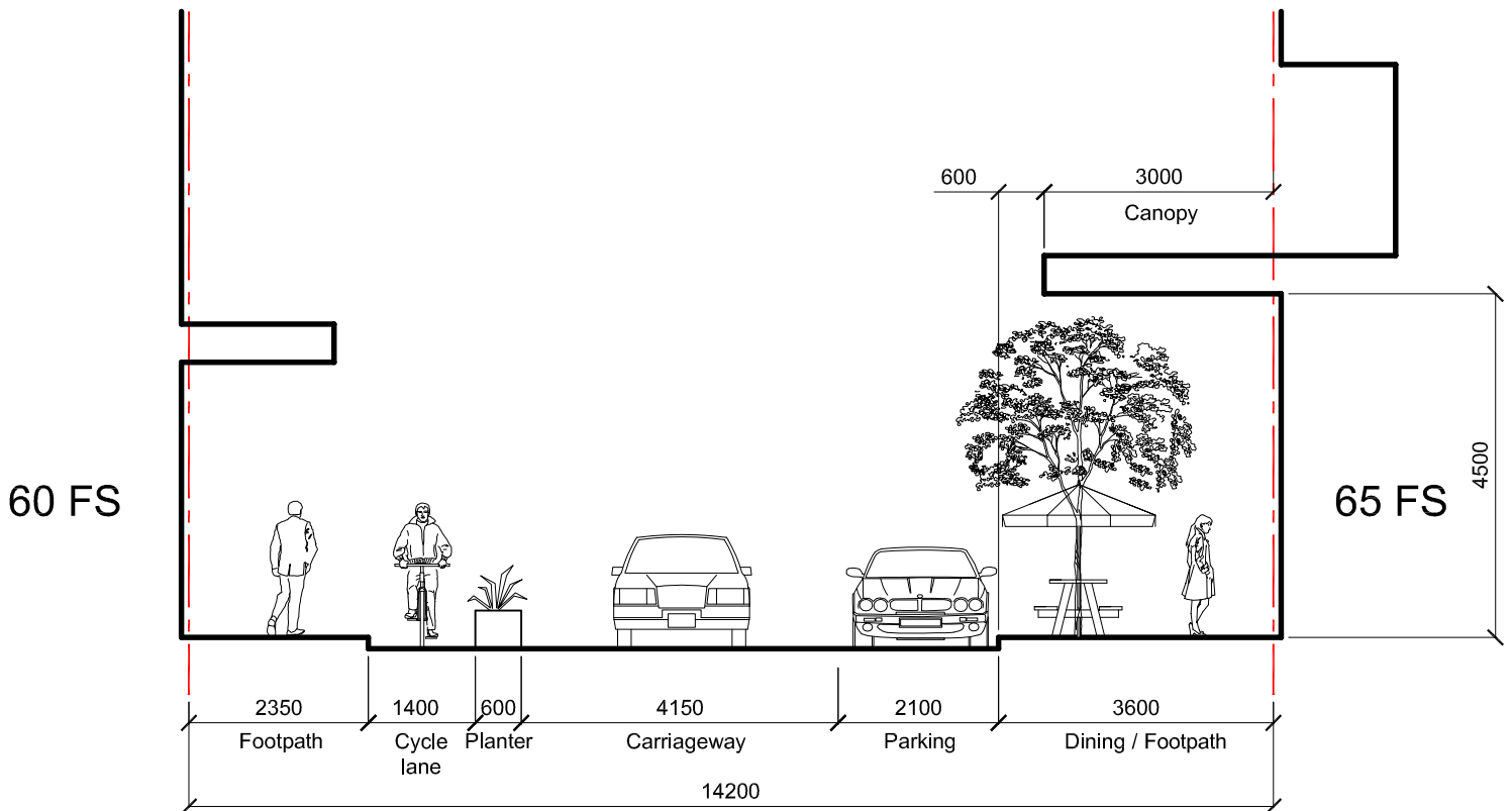
2 Updated Baseline Streetscape Upgrade and Proposed Building
