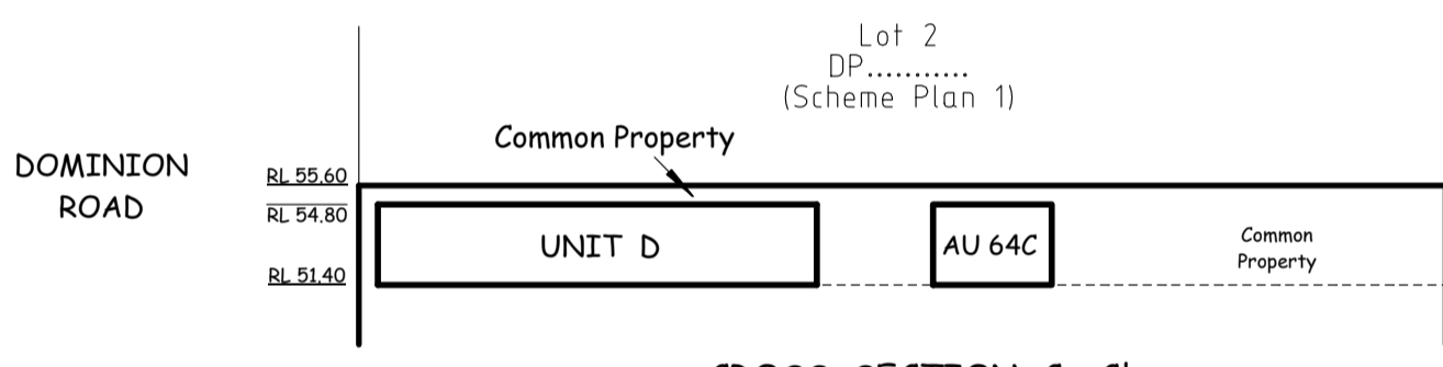
CROSS SECTION C - C'
