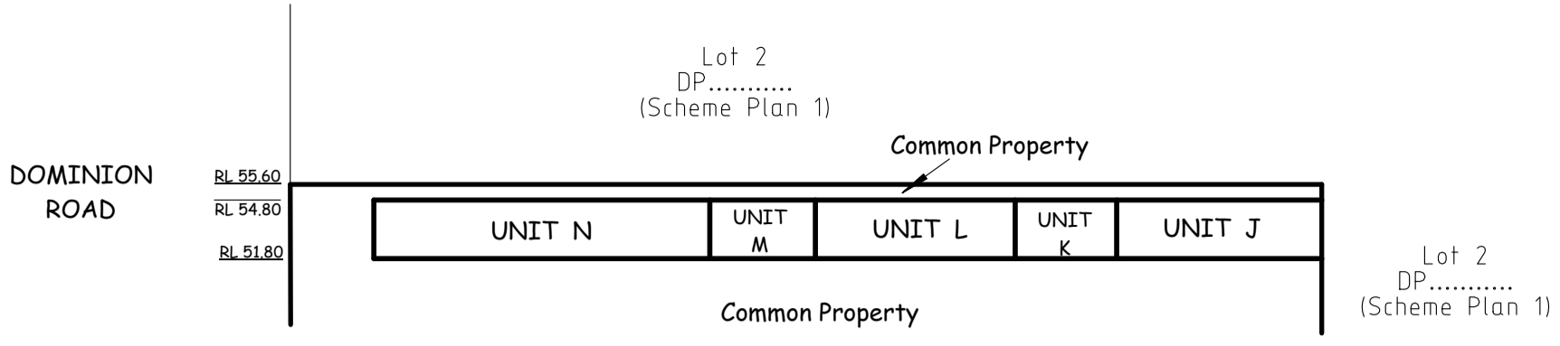
CROSS SECTION A - A'
